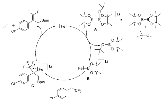
Scheme 3. Gram-Scale Reaction
